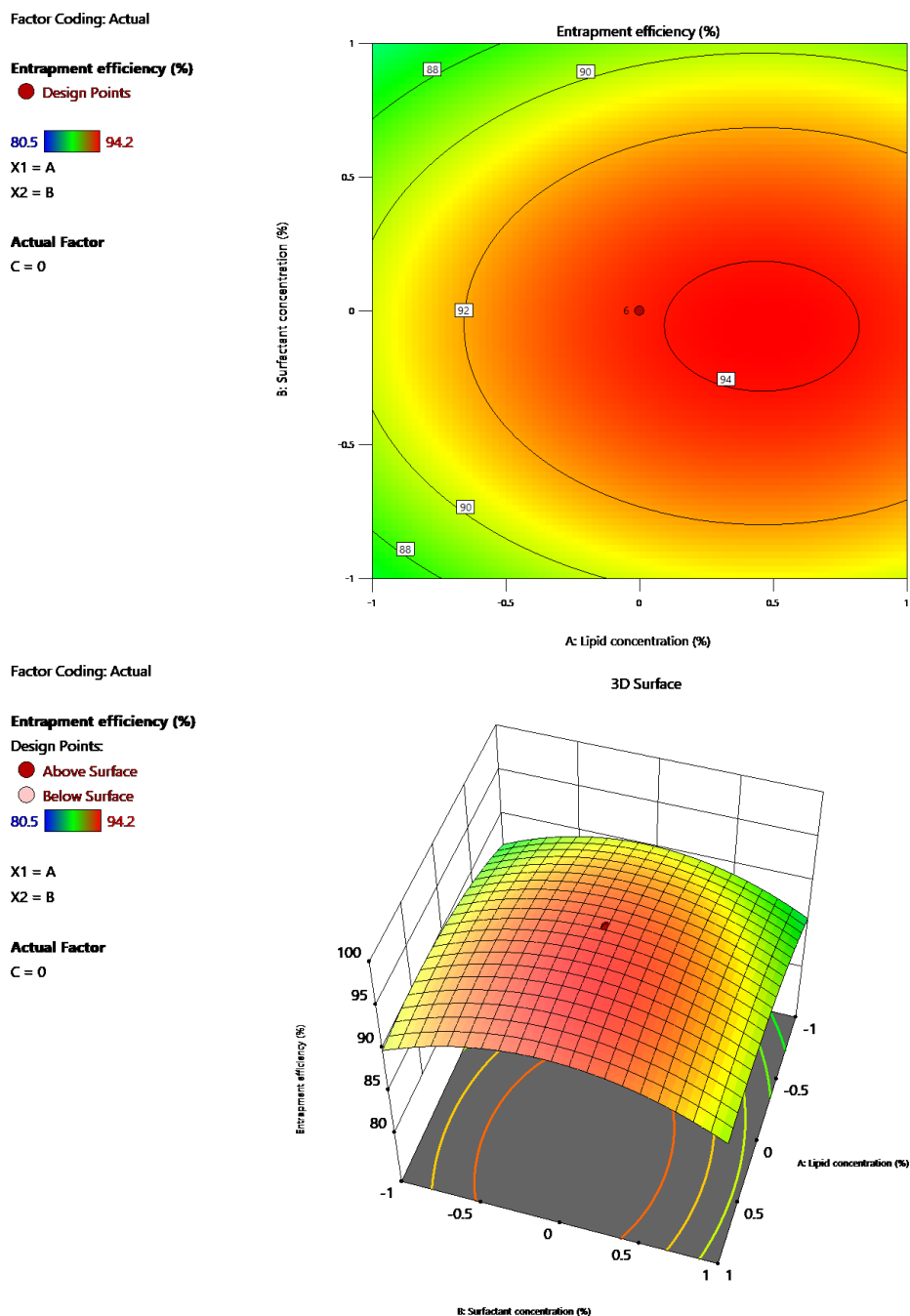
Figure 5: Contour Graphs and 3D Surface Graphs of Particle Size (nm) and Entrapment Efficiency (%).
