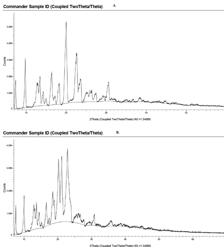
Figure 4: In vitro Drug Release, SEM of Optimized Batch and XRD A) Pure Drug, B) Prepared SLN.
